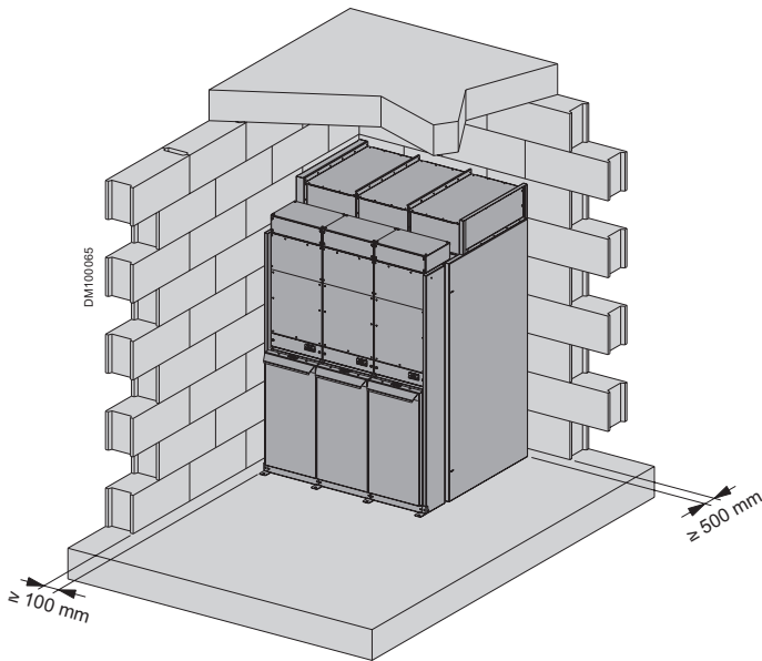
顶部泄压内燃弧开关柜的布置
